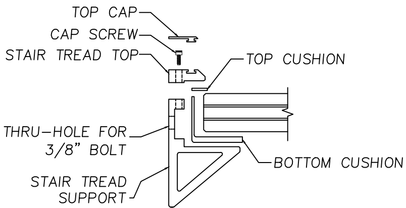
STAIR TREAD SUPPORT BRACKET ASSEMBLED VIEW
