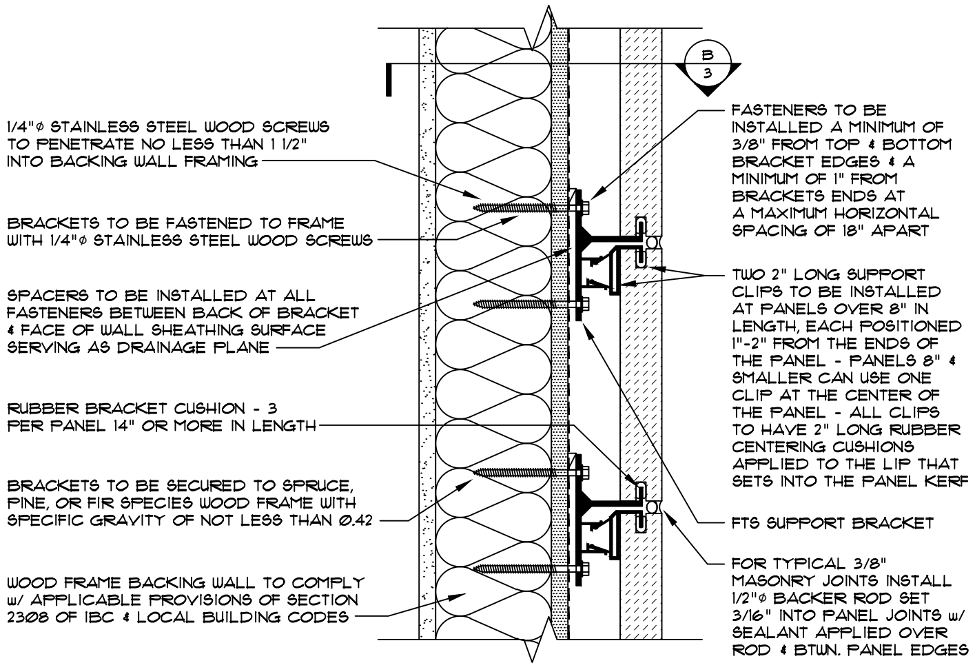
MID WALL - SECTION VIEW A-3
