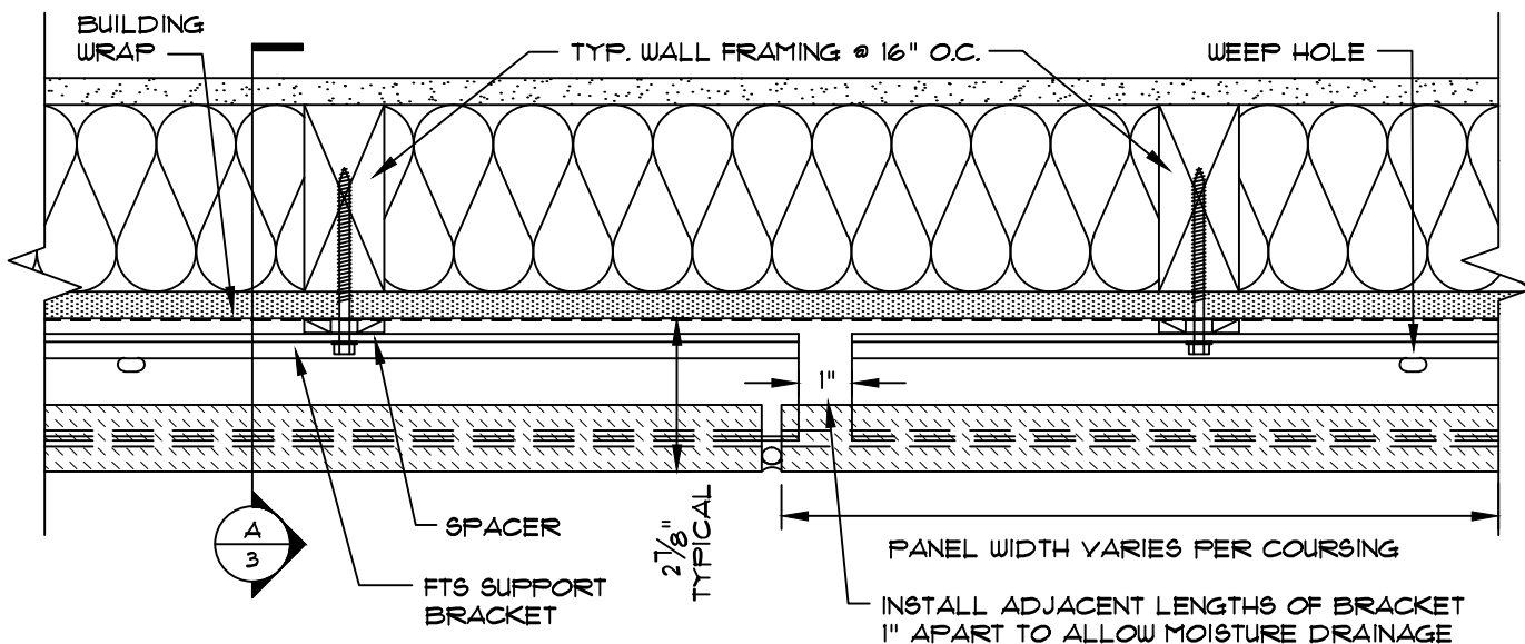
MID WALL - PLAN VIEW B-3
